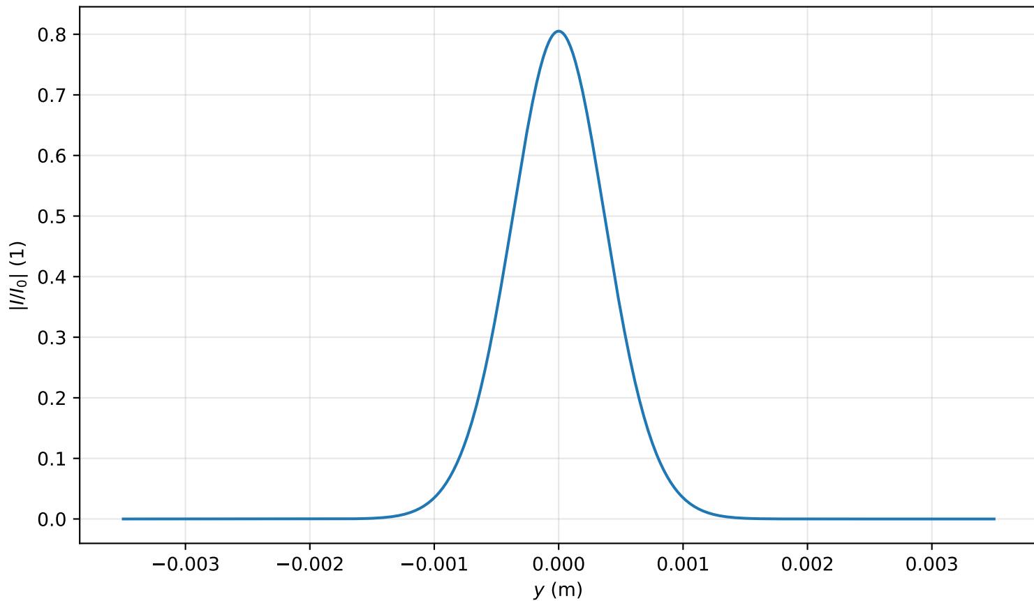
Intensity profile I(x=0, y, z=1.274)/I_0 , P_{in}=0.2P_{cr} , artificial time
